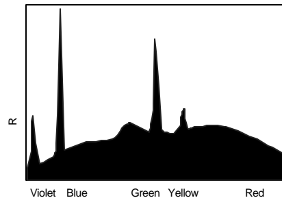
Fig. 2 - SPD of 5000K Fluorescent Source
